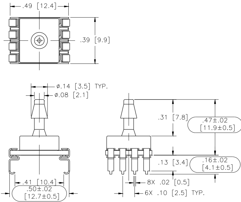
Model: MS4525DO-TPvoixxyS
